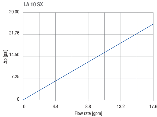
FLOW RATE vs PRESSURE DROP Δp | - Testing mode: 68°F - 43.5 psi (20°C - 3 bar)
