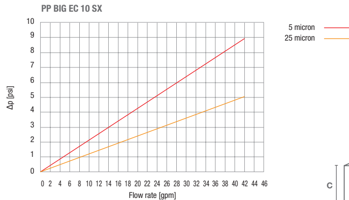
FLOW RATE vs PRESSURE DROP Δp | - Testing mode: 68°F - 43.5 psi (20°C - 3 bar)
