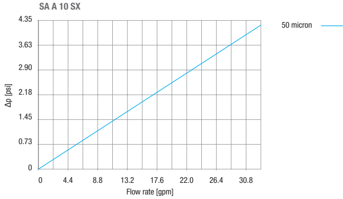
FLOW RATE vs PRESSURE DROP \Delta p | - Testing mode: 68°F - 43.5 psi (20°C - 3 bar)
